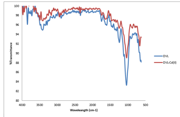
Figure 1. FTIR spectra of DVL before and after adsorption of Cd(II) ions
