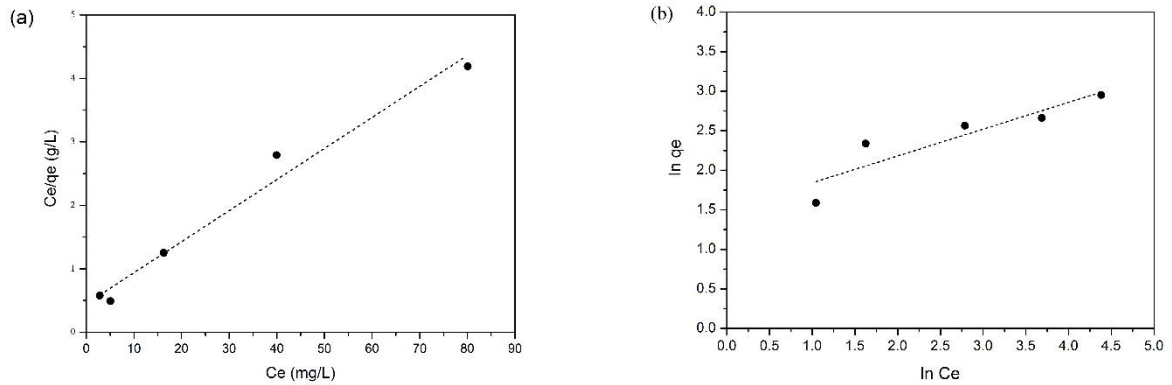
Figure S2. Isotherm plots for adsorption of MB on CFMo; (a) Langmuir isotherm model and (b) Freundlich isotherm model
