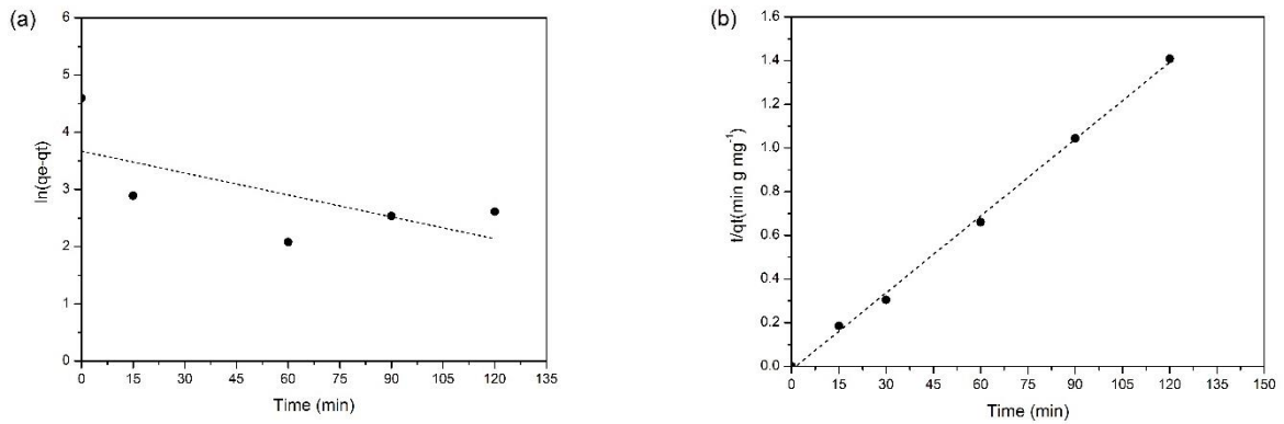
Figure S1. Adsorption kinetic for removal of MB on CFMo: (a) pseudo-first order and (b) pseudo-second order models
