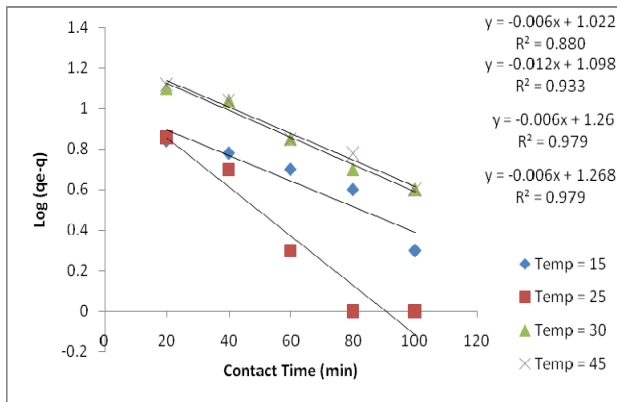
Figure 21: Plots of \log (q_e - q) versus time for Cu^{2+} ion adsorption onto CAC
