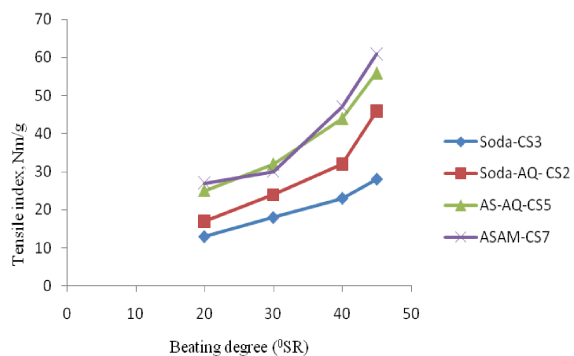
Fig. 3: Tensile index vs. beating degree (°SR) of Gossypium hirsutum unbleached pulps
