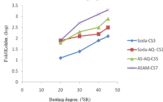
Fig. 6: Fold Kohler vs. beating degree (°SR) of Gossypium hirsutum unbleached pulps
