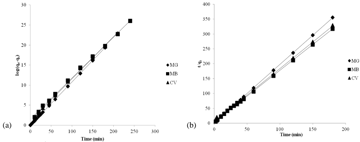
Fig. 6: Pseudo 2 nd Order Kinetics (a) Single System (b) Tertiary System
