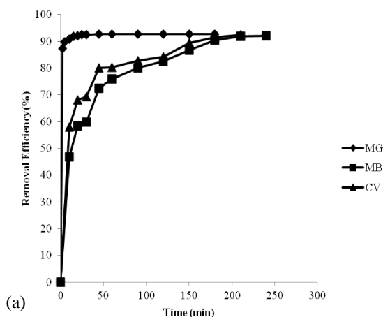
Fig. 4: Effect of Contact Time (a) Single System (b) Tertiary System
