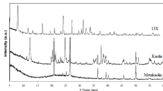
Figure 1. XRD pattern of kaolin, metakaolin and commercial zeolite 13X
