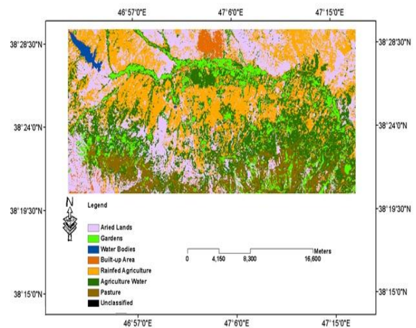
Figure 5. The developed land use land cover map for 2010
