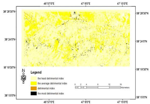
Figure 7. The detrimental index map from 1987 to 2010
