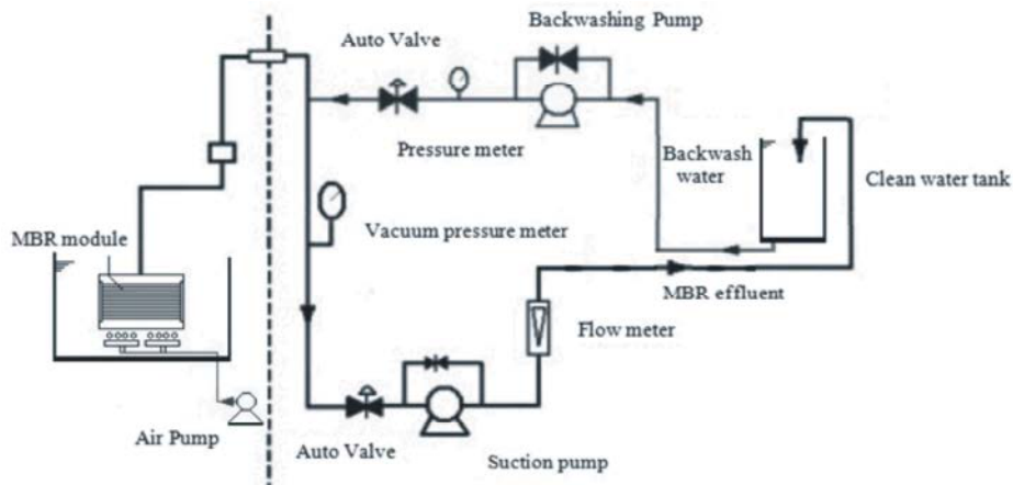
Fig. 1: NF-MBR pilot plant schematic
