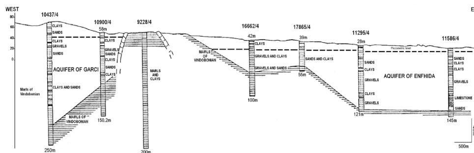
Fig. 2: Longitudinal section through the aquifer of El Khairat (Mena et al. , 1996).
