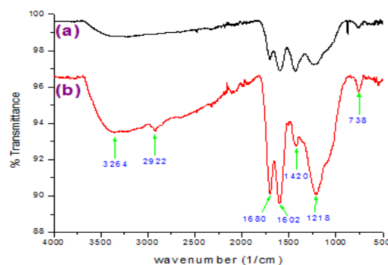
Figure 11. FT-IR spectra for a) PJP and b) dye loaded PJP
